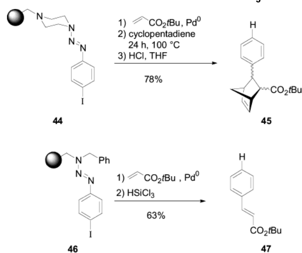
Scheme 7. The T1 Linker for Traceless Cleavage
